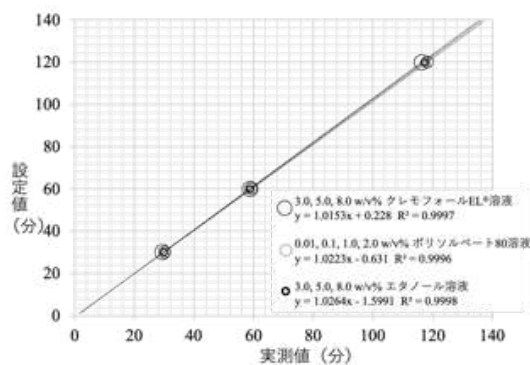
Fig. 9. Influence on the administration rate of the peristaltic finger infusion pump by using pharmaceuticals containing surfactants and ethanol
